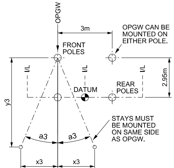
PLAN VIEW SHOWING TOP STAY SPLAY ANGLES
